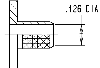
CRIMP SLEEVE
